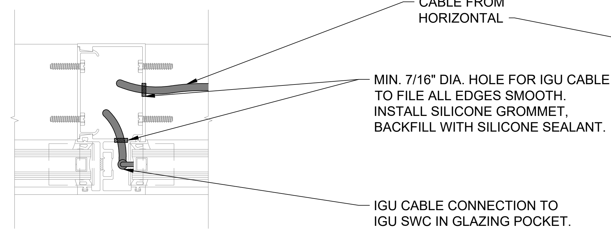
DETAIL 5 VERTICAL MULLION
