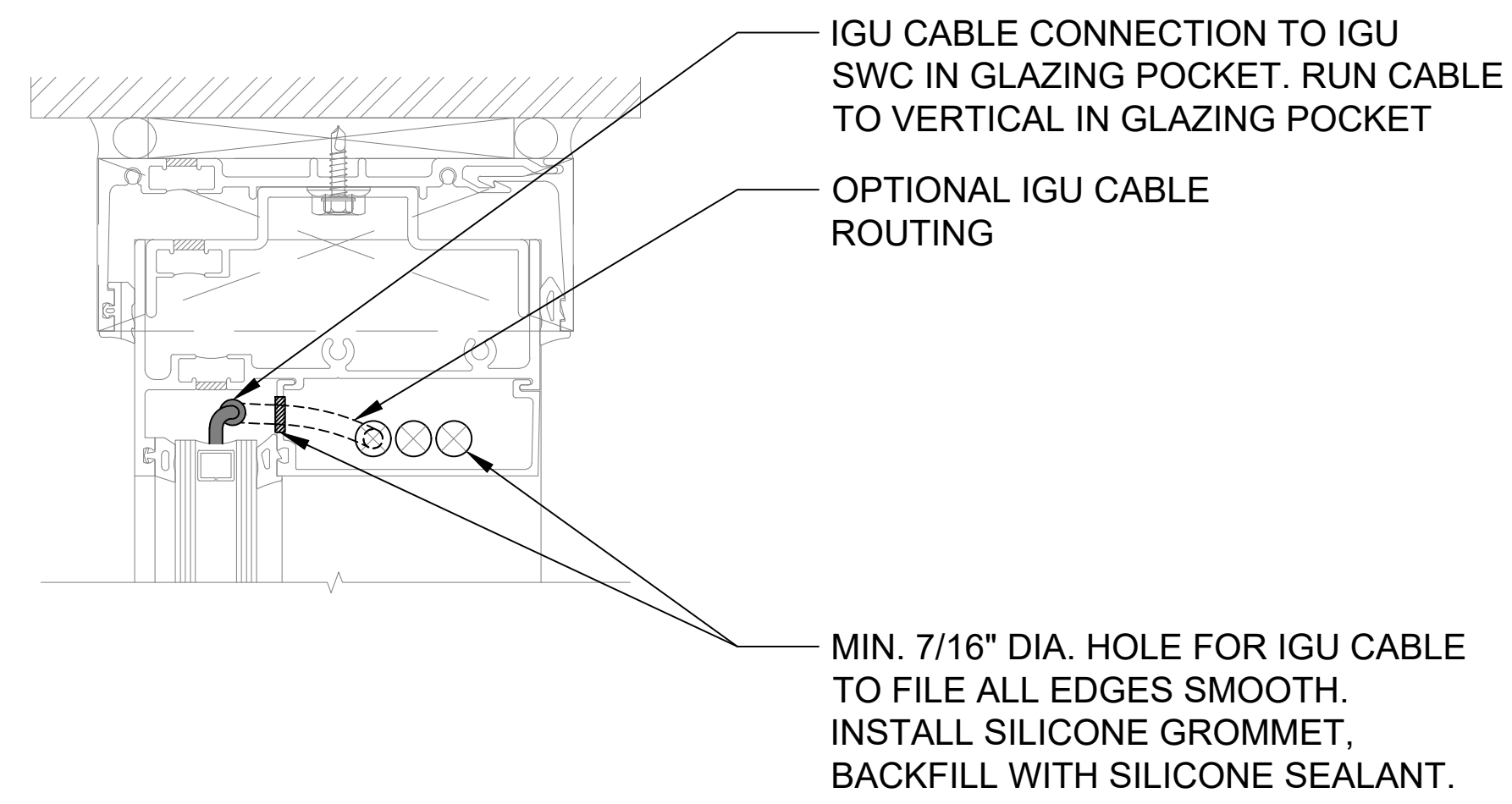
DETAIL 1 HEAD
